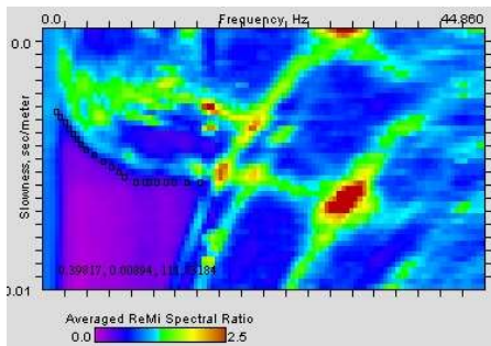
typical Remi spectrum and DC curve (48ch, 5m spacing)
